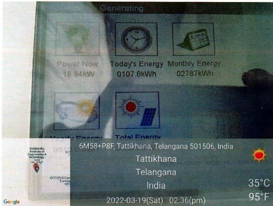
Wheeling to grid metering arrangement with display.
